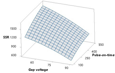
(b) SSR vs. gap voltage, pulse-on time
