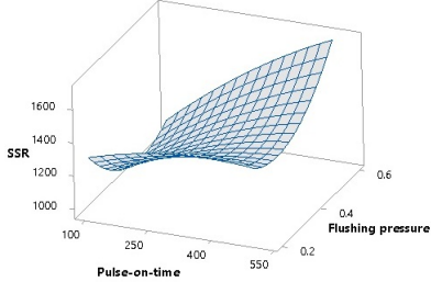
(i) SSR vs. pulse-on time, flushing pressure
