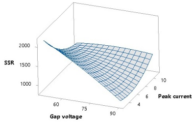
(a) SSR vs. gap voltage, peak current
