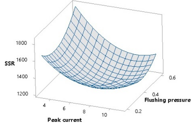
(g) SSR vs. peak current, flushing pressure
