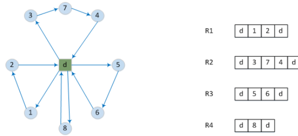
Figure 1: initial Solution
