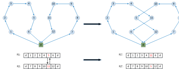
Figure 5: Inter-route Permutaion
